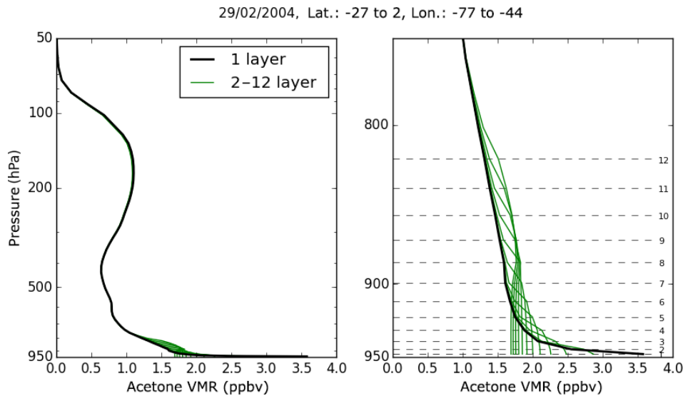
Figure 5. Profiles of the acetone VMR for n_{\text{lev,emi}} = 1 (emission height of 20 m above ground, black thick) and 2 to 12 (emission height of 65 to ~ 1500 m above ground, green thin lines) spatially averaged over the Amazon region in Brazil on 29 February 2004, about two months after initialisation. In the right panel, the pressure range is reduced and the average height of the 12 lowest model layers are illustrated by the dashed horizontal lines.
