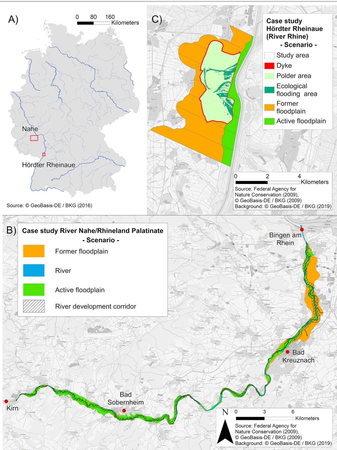
FIGURE 2 | (A) Map of federal states and rivers in Germany. The two case studies are localized by red boxes. (B) Case study River Nahe: floodplain compartments active (light green) and former (orange) floodplain, river (blue), and area for the water development corridor (black striped area) of the scenario. River floodplain corridor = the area potentially available for the restoration of rivers and its floodplains in order to bring them into a good or very good ecological status. Red dots indicate larger towns. (C) Case study Hördter Rheinaue along the River Rhine: floodplain compartments active (light green) and former (orange) floodplain and river (blue). Dyke (red) and polder area (light green area) of the scenario.
