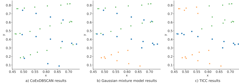
Figure 6. Comparison of clustering algorithms on the LIBRAS dataset on an individual sample from the vertical zigzag class (see sample 123 from Figure 5); a) CoExDBSCAN results (points labeled as noise are omitted), b) GMM results, and c) TICC results.
