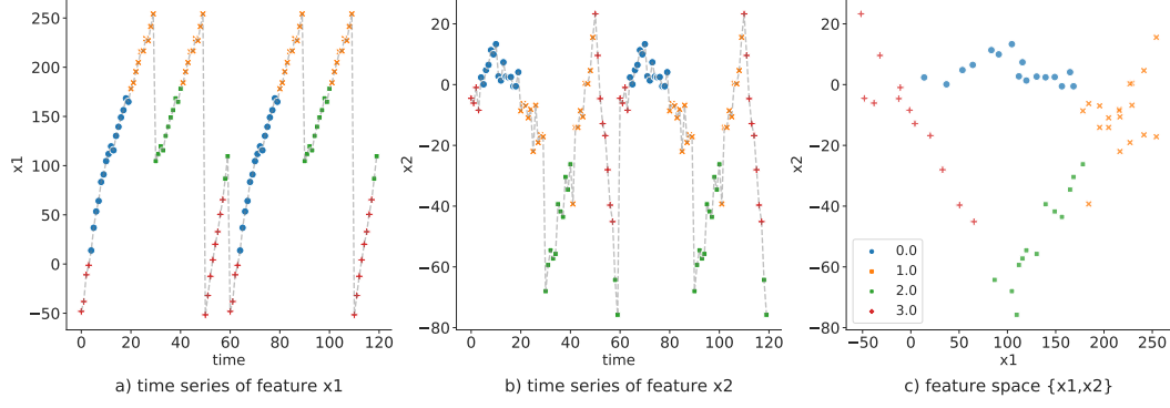
Figure 2. Time point clustering with the TICC algorithm; a) time series for feature x_1 with predicted labels, b) time series for feature x_2 with predicted labels and c) joint feature space \{x_1, x_2\} with predicted labels.
