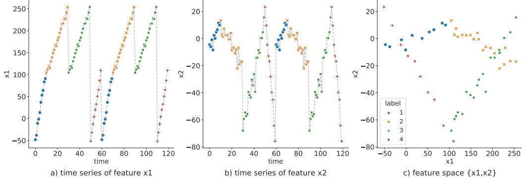
Figure 1. Synthetic dataset; a) time series for feature x1, b) time series for feature x2 and c) joint feature space \{x1, x2\} . Labels are true labels.
