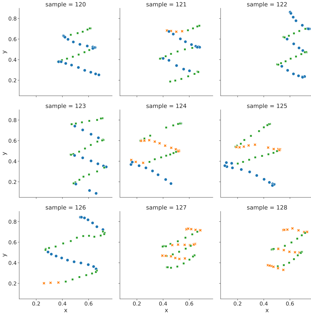
Figure 5. Semi-supervised time point clustering with the modified CoExDBSCAN algorithm on the LIBRAS dataset. Nine samples from one class (vertical zigzag) illustrate the successful segmentation of each time series into similar motions.
