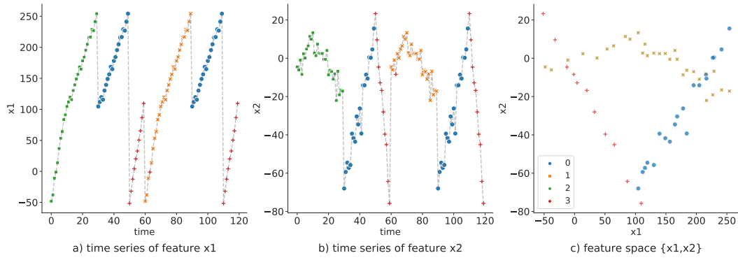
Figure 3. Time point clustering with the Gaussian mixture model ( GMM ); a) time series for feature x_1 with predicted labels, b) time series for feature x_2 with predicted labels and c) joint feature space \{x_1, x_2\} with predicted labels (orange crosses and green squares are overlaid).
