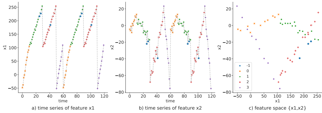
Figure 4. Semi-supervised time point clustering with the modified CoExDBSCAN algorithm; a) time series for feature x_1 with predicted labels, b) time series for feature x_2 with predicted labels and c) joint feature space \{x_1, x_2\} with predicted labels.
