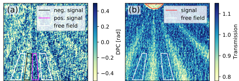
Figure 2. Reconstructed DPC (a) and transmission image (b) using the reference image one. Although the Moiré stripes are completely removable, the image is still noisy due to the low photon flux. The colored boxes mark the regions of interest (ROI) which are used for the evaluation process of the image.
