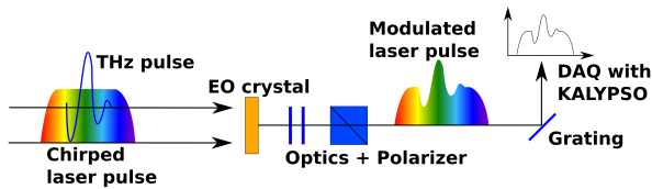
Figure 2: Principle of EOSD of a THz pulse with a chirped laser pulse: THz and laser pulse are overlapped collinearly in the EO crystal. The electrical field of the THz pulse generates a modulation in the intensity of the laser pulse spectrum, which can be analyzed in a spectrometer.
