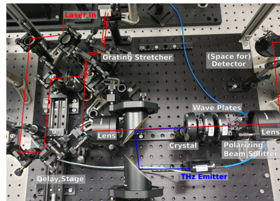
Figure 3: Picture of the optical setup of the EOSD far-field demonstrator. The laser beam path is shown in red, the THz beam path in blue. In this configuration a commercial spectrometer is integrated for diagnostics, during the EOSD measurements an optical spectrometer with KALYPSO as detector is integrated.
