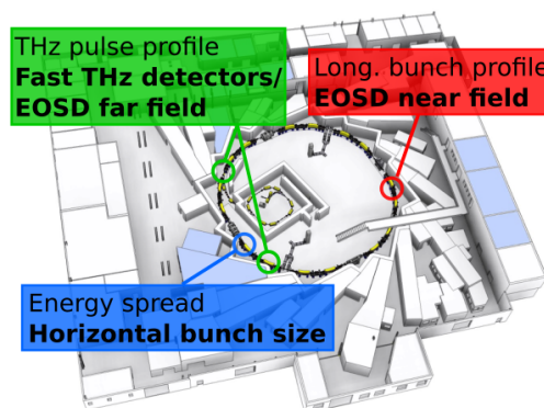
Figure 1: Location of a selection of sensors of the distributed sensor network at KARA.
