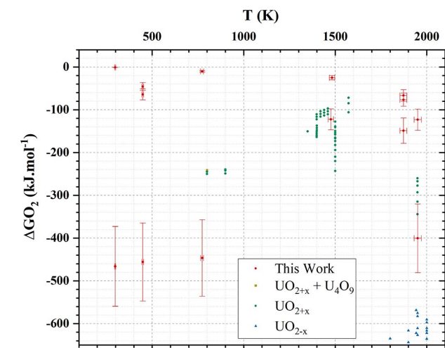
Figure 4 Oxygen potential ( \text{kJ mol}^{-1} ) and temperature (K) of our experimental data and the experimental U–O thermodynamic data selected by Guéneau et al. (2011). Note that only bibliographic data corresponding to the range of our study have been plotted.
