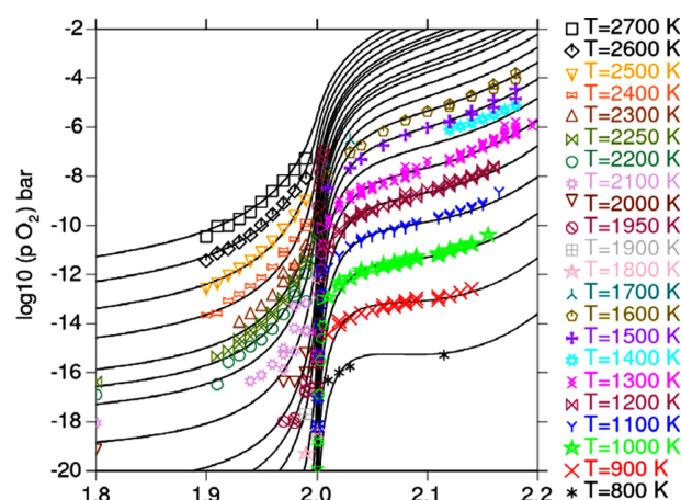
Figure 3 Oxygen activities in \text{UO}_{2\pm x} calculated (black line) with selected experimental data (coloured symbol) from Guéneau et al. (2011). Reprinted from Guéneau et al. (2011), Copyright (2011), with permission from Elsevier.
