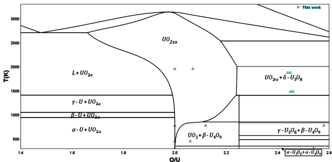
Figure 6 Our experimental point (blue triangles) in the calculated U–O phase diagram.
