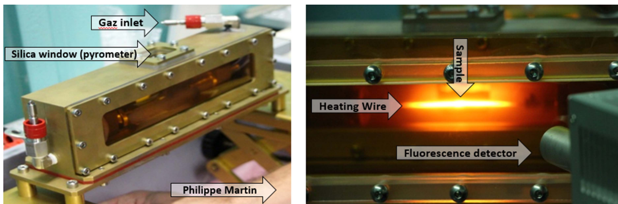
Figure 2 Photographs of the heating setup.
