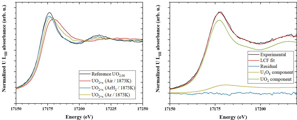
Figure 5 (a) U L_{\text{III}} XANES spectra of \text{UO}_{2+x} samples measured at 1873 (19) K in different oxygen potentials. (b) LCF of a U L_{\text{III}} XANES experimental spectrum fitted with \text{UO}_2 and \text{U}_3\text{O}_8 components.
