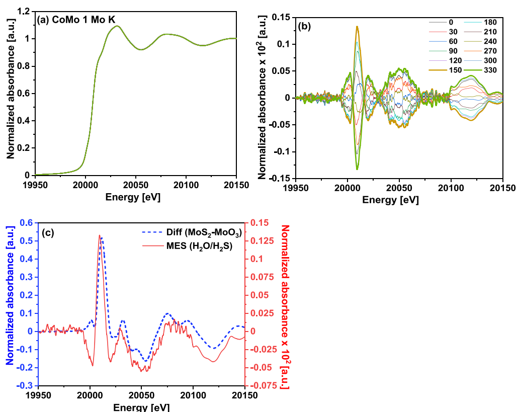
Figure 3. (a) Normalized, time-resolved Mo K-edge XANES consisting of a total of 36 spectra covering 10 s each for the CoMo 1 catalyst during 3% \text{H}_2\text{O}/\text{H}_2 (0–180 s) vs 500 ppm \text{H}_2\text{S}/\text{H}_2 (180–360 s) cycling and 10 period average. (b) Corresponding demodulated spectra at selected values of phase angle ( \Delta\phi ). (c) Comparison of the ( \text{MoS}_2 - \text{MoO}_3 ) difference spectrum (blue dashed line) with the maximum amplitude signal obtained at \Delta\phi = 150^\circ after demodulation (red line) for the CoMo 1 catalyst.
