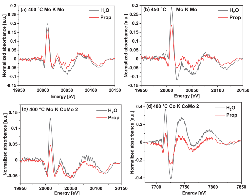
Figure 12. Comparison of the maximum amplitude of the demodulated spectra obtained from the two different cycling experiments \text{H}_2\text{O} vs \text{H}_2\text{S} and 1-propanol vs \text{H}_2\text{S} (inlet position of the quartz microreactor) at the Mo K-edge for (a) Mo at 400 °C, (b) Mo at 450 °C, (c) CoMo 2 at 400 °C, and (d) at the Co K-edge for CoMo 2 at 400 °C.
