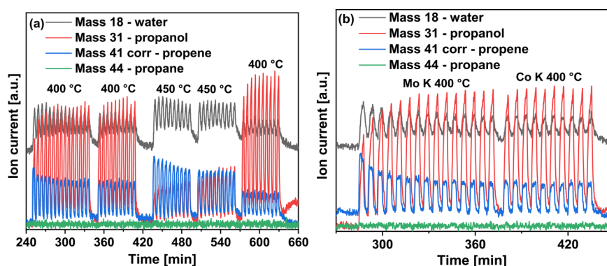
Figure 9. MS signal during 1-propanol/ \text{H}_2 - \text{H}_2\text{S} / \text{H}_2 cycling for (a) the Mo catalyst where a total of five MES experiments were performed at the Mo K-edge focusing the X-ray beam at the inlet and outlet positions of the quartz microreactor at 400 and 450 °C and (b) the CoMo 2 catalyst where two MES experiments were performed, one at the Mo K-edge and another at the Co K-edge, both focusing the X-ray beam at the inlet position of the microreactor at 400 °C. The MS signal encompasses the activity of the entire catalyst loaded in the microreactor.
