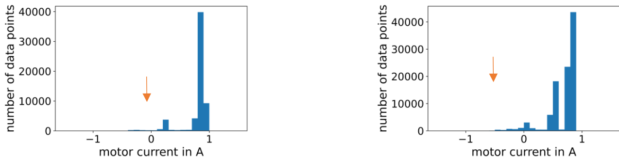
Figure 6. Histogram of training data over motor current generated while milling with tool diameter 10 mm ( left ) and tool diameter 8 mm ( right ). In the right image, a shift to the left is noticeable as well as a peak at 0.5 which results from one tool path with reduced radial depth of cut.
