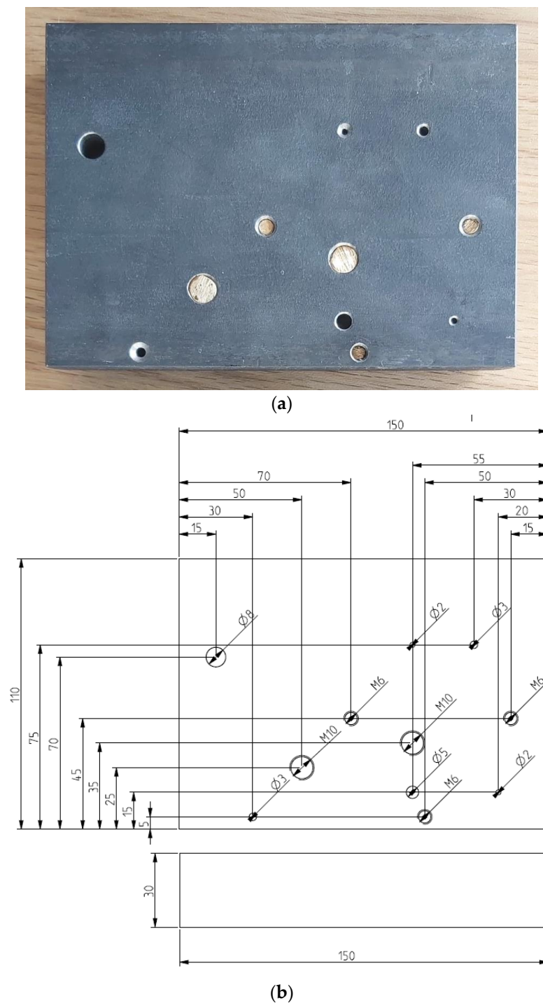
Figure 1. Top view of the workpiece with artificially inserted anomalies in the form of boreholes and brass (a) and its dimensions in mm (b).
