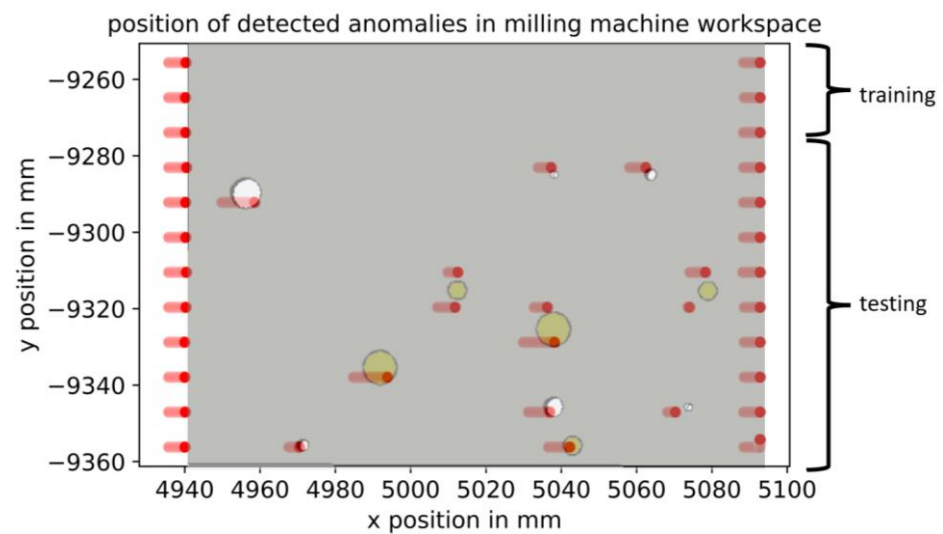
Figure 5. Workpiece with artificially inserted anomalies in the form of boreholes and brass and detected anomalies (red).
