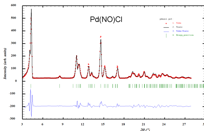
Figure 6. Rietveld plot of the Guinier diffractogram for \text{PdCl}(\text{NO}) , obtained at 298 K using \text{MoK}\alpha_1 radiation in the 2\theta -range from 3 – 28^\circ with increment 0.04^\circ .
