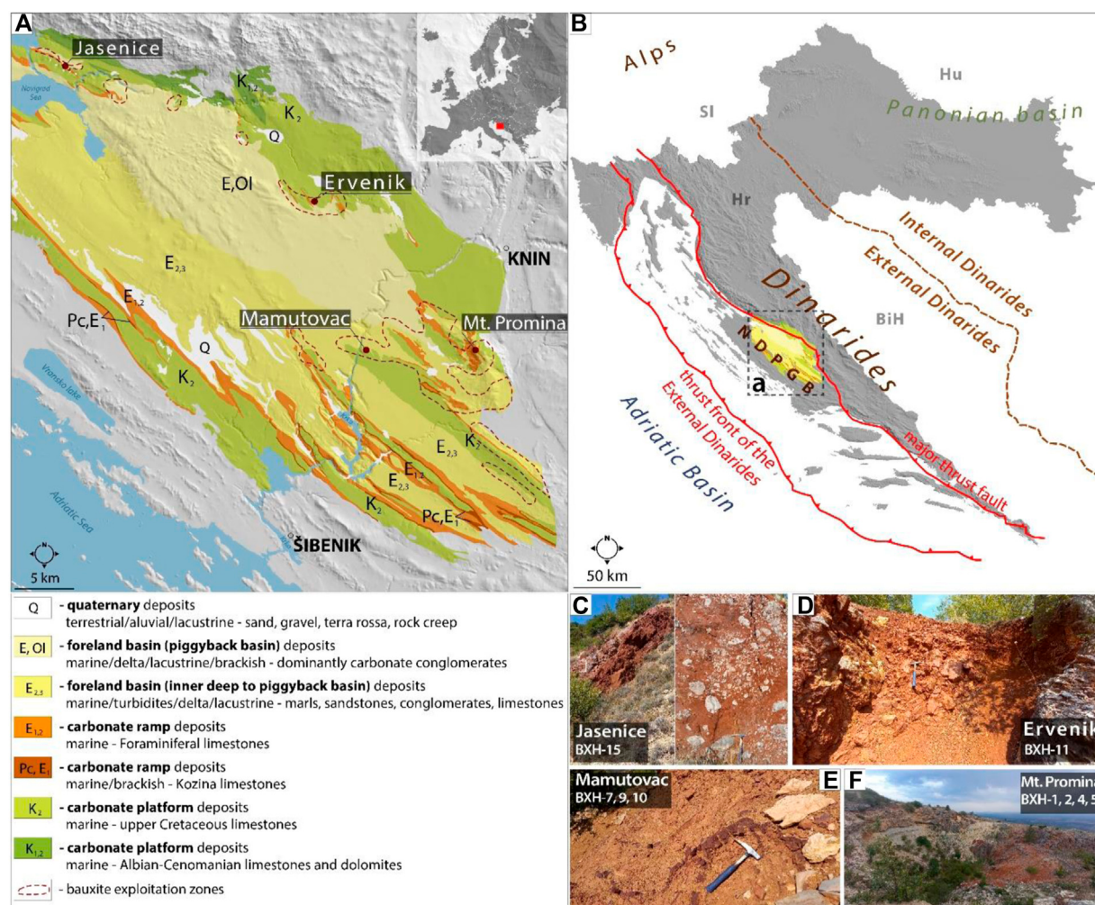
FIGURE 1 (A) Geological map of the study area (modified according to the work of Mamužić (1971), Ivanović et al. (1973), Ivanović et al. (1976), and Ivanović et al. (1977)) with indicated major units of the North Dalmatian foreland basin, bauxite exploitation zones, and sampling positions; (B) location of the North Dalmatian piggyback basin as part of the wider foreland basin with respect to the major thrust fault system in the External Dinarides (Basic Geological Map of the Republic of Croatia 1:300,000); (C) Jasenice sampled outcrop; (D) Ervenik sampled outcrop; (E) Mamutovac sampled outcrop; and (F) Mt. Promina sampled outcrop.
