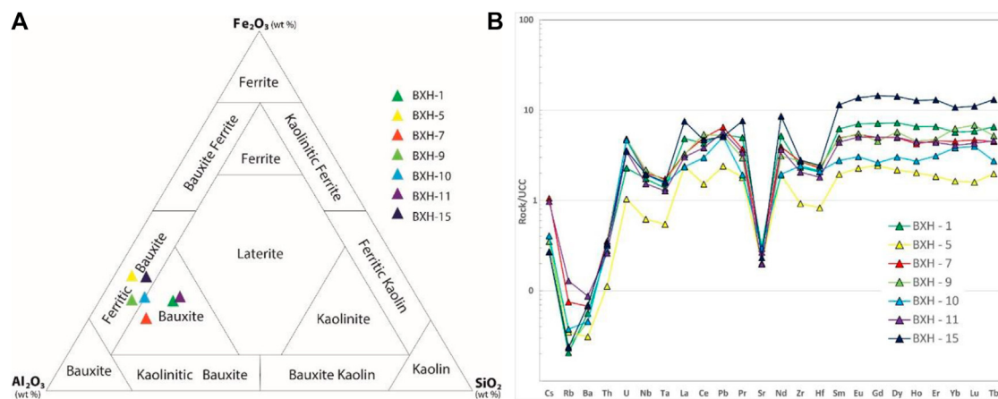
FIGURE 8 (A) Whole-rock compositions of BXH samples on a three-component diagram (Aleva, 1994) and (B) upper continental crust-normed spider diagram comparing the trace element geochemistry of the bauxite samples.
