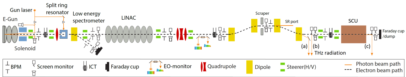
Figure 1: Schematic layout including beam diagnostics and proposed position of superconducting undulator (SCU), not to scale. (a) CSR/CER, (b) CTR, (c) radiation from SCU.
