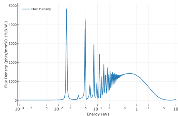
Figure 2: Spectrum of the spacial flux density produced by the ideal THz undulator at FLUTE with SPECTRA [9] on-axis at 1 m distance with 0.1 nC bunch charge.
