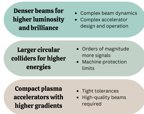
Figure 2: Some trends and related challenges of frontier accelerators.
