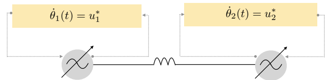
Fig. 1. Two-inverter system in closed-loop with angular droop (19).
