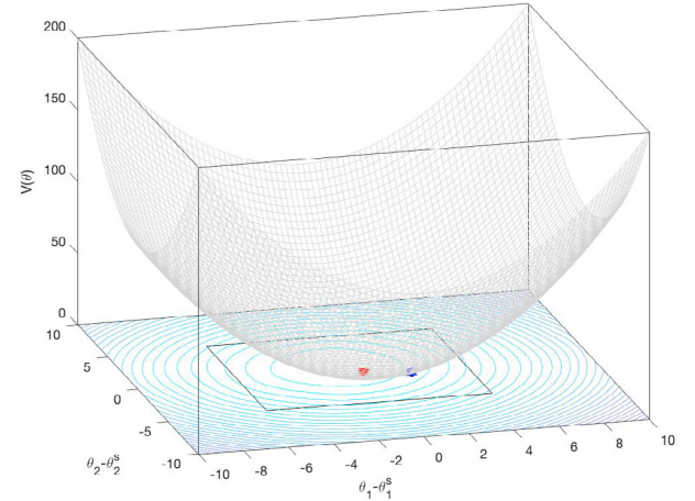
Fig. 4. 3-D Representation of the sublevel set of the Lyapunov function V in (17) in blue and the state constraint set \mathcal{X} in (15) in black containing the origin marked by the red star. The initial condition \theta_0 \in \mathcal{X} marked by the blue star is chosen such that the set \Omega_c in (6) is contained in the box \mathcal{X} .
