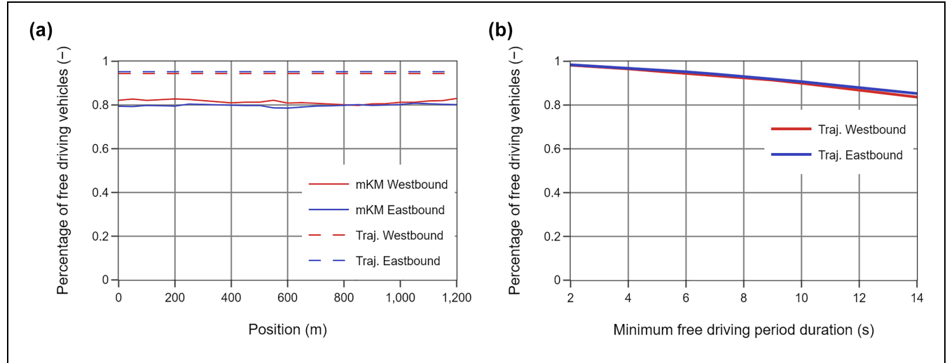
Figure 10. Percentage of free driving passenger cars depending on the used approach (a) and the min. free driving period duration (b).
