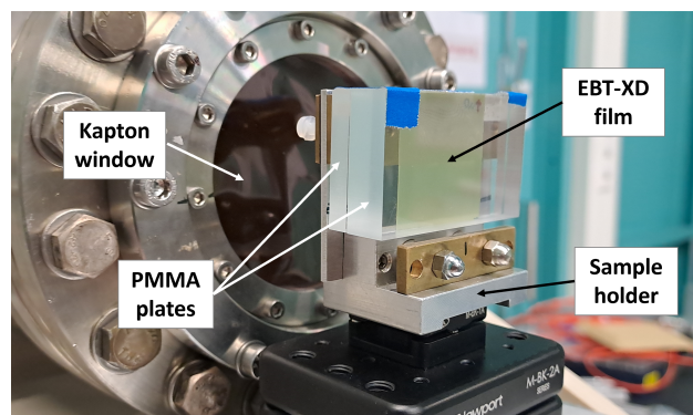
Figure 4: EBT-XD irradiation setup at the IMAGE X-ray beamline at the synchrotron KARA. Films placed between PMMA plates serve as a water phantom substitute.
