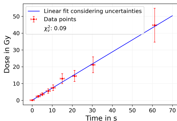
Figure 6: Measured dose at the IMAGE X-ray beamline at KARA. On the ordinate, the average dose D per EBT-XD film is plotted against the corresponding film exposure time t on the abscissa.
