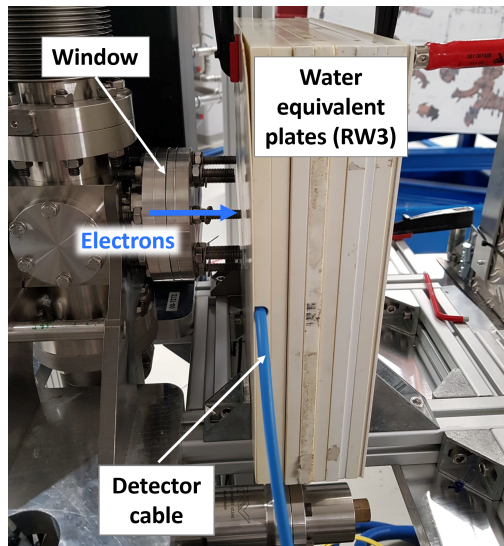
Figure 2: Depth dose curve measurement setup at FLUTE. The electrons pass through a 150 \mu\text{m} stainless steel window into air, where they then traverse a water phantom with the embedded detector.
