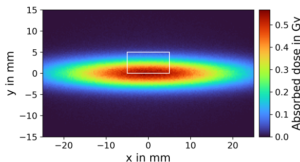
Figure 7: Simulated 2D absorbed dose profile for an exposure time of t = 11 \text{ s} and a photon beam with Gaussian shape and an energy of 16 keV.
