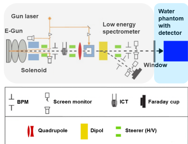
Figure 1: Schematic low energy section setup of FLUTE. The section with ultra-high vacuum ( 10^{-9} mbar) is marked in light gray and the section with ambient air in light blue. Adapted from [10].
