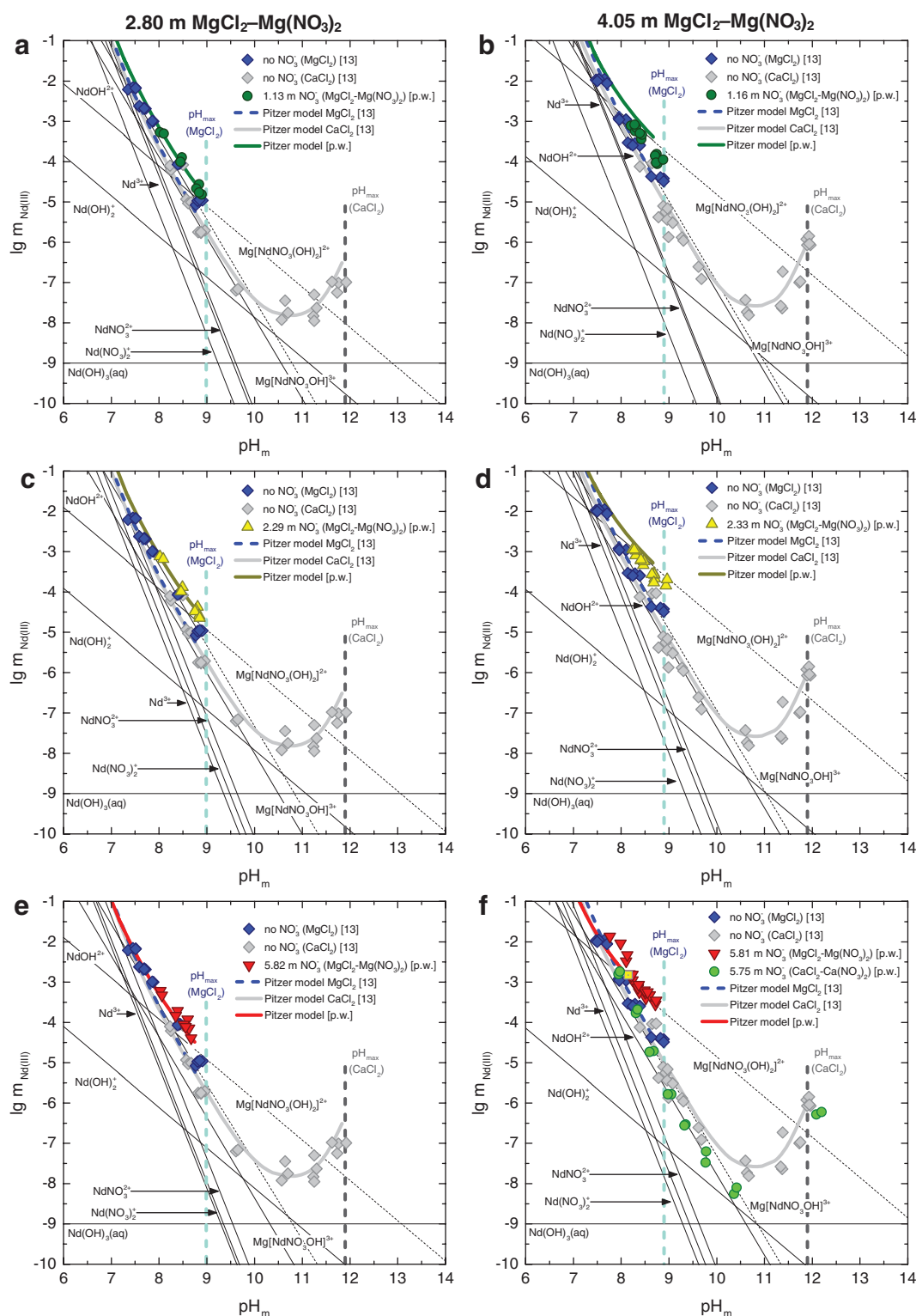
Fig. 3: Solubility of \text{Nd(OH)}_3(\text{s}) in 2.80\text{ m MgCl}_2\text{--Mg(NO}_3)_2 with (a) 1.13\text{ m} , (c) 2.29\text{ m} and (e) 5.82\text{ m NO}_3^- in comparison with 4.05\text{ m MgCl}_2\text{--Mg(NO}_3)_2 with (b) 1.16\text{ m} , (d) 2.33\text{ m} and (f) 5.81\text{ m NO}_3^- . The solubility data of \text{Nd(OH)}_3(\text{s}) in 4.02\text{ m CaCl}_2\text{--Ca(NO}_3)_2 with 5.75\text{ m NO}_3^- are also included in figure (f). Reference data in nitrate-free solutions [13] is included in all the figures for comparison. Yellow square in (f) indicates the sample used for Nd–L III EXAFS measurements. Thick solid lines correspond to the \text{Nd(III)} solubility calculated using thermodynamic and activity models: for pure \text{MgCl}_2 and \text{CaCl}_2 systems (blue and grey lines) [13]; for \text{MgCl}_2\text{--Mg(NO}_3)_2 mixtures (green, yellow, red lines) [p.w.]. Thin lines show the aqueous speciation underlying \text{Nd(OH)}_3(\text{s}) solubility curve in \text{MgCl}_2\text{--Mg(NO}_3)_2 systems.
